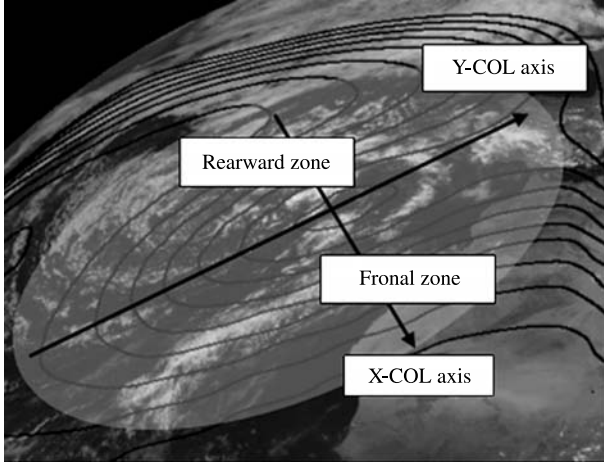
Fig. 5. VIS Image 16-06-95 at 12:00 UTC, showing the COL-axes system. The Y-COL-axis divides the entire area in two regions: the rearward and the frontal zone. In this case COL-axes system coincides with the asymmetric ellipse axes
