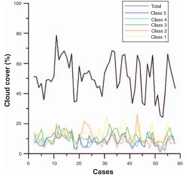
Fig. 6. Averaged values of whole cloud area (WCA) in the COL selected area for each studied cases. Red colour represents low clouds and yellow mid-level clouds
