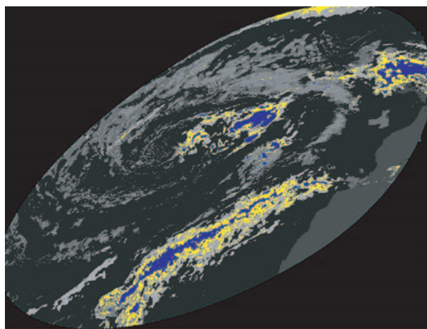
Fig. 7. VIS Image 16-06-95 at 12:00 UTC showing high clouds (in yellow) and deep convection clouds (in blue). The high correlation between these types of clouds is clear in this figure
