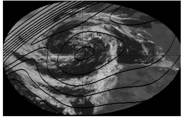
Fig. 10. VIS Image 04-08-95 at 12:00 UTC showing closed cyclonic circulation during the third stage of a COL-system
