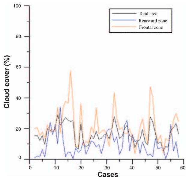
Fig. 8. Averaged values of WCA, RWCA and FWCA for high and deep convective clouds for each studied cases. High and deep convective clouds has a major presence in the frontal zone of the COL selected area
