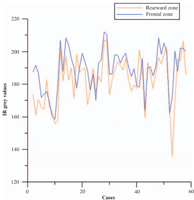
Fig. 12. Average values of IR brightness counts for the rearward and frontal zones for each studied case. Higher values in the frontal zone indicate cooling in this zone
