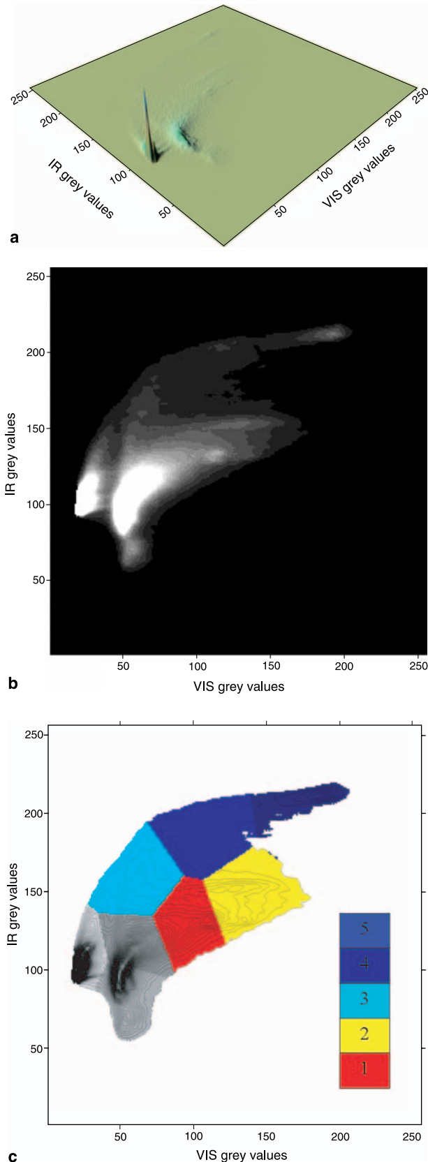
Fig. 2. Bispectral histogram in a 3D (a) and 2D (b) representation and classified results: Dark blue (C5), blue (C4), light blue (C3), yellow (C2) and red (C1) (c). The region of grey colour corresponds to land and sea
