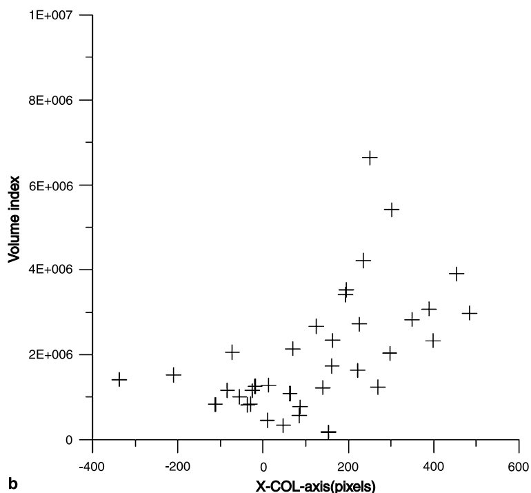
Fig. 13. Average values of the Volume index for high and deep convective clouds versus X-COL coordinates (in pixels) for each studied case (a), first stage cases (b), second stage cases (c), third stage cases (d), cold season cases (e) and hot season cases (f). The positive X-COL axis represents the frontal zone. Higher values of Volume index in this zone indicate major probability of heavy rainfalls
